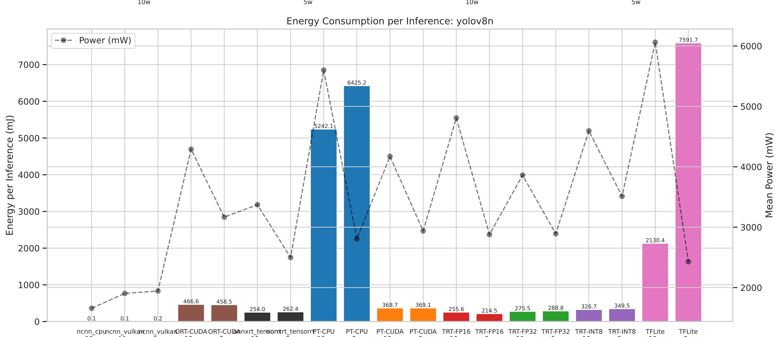
Energy Consumption per Inference: yoloV8n
