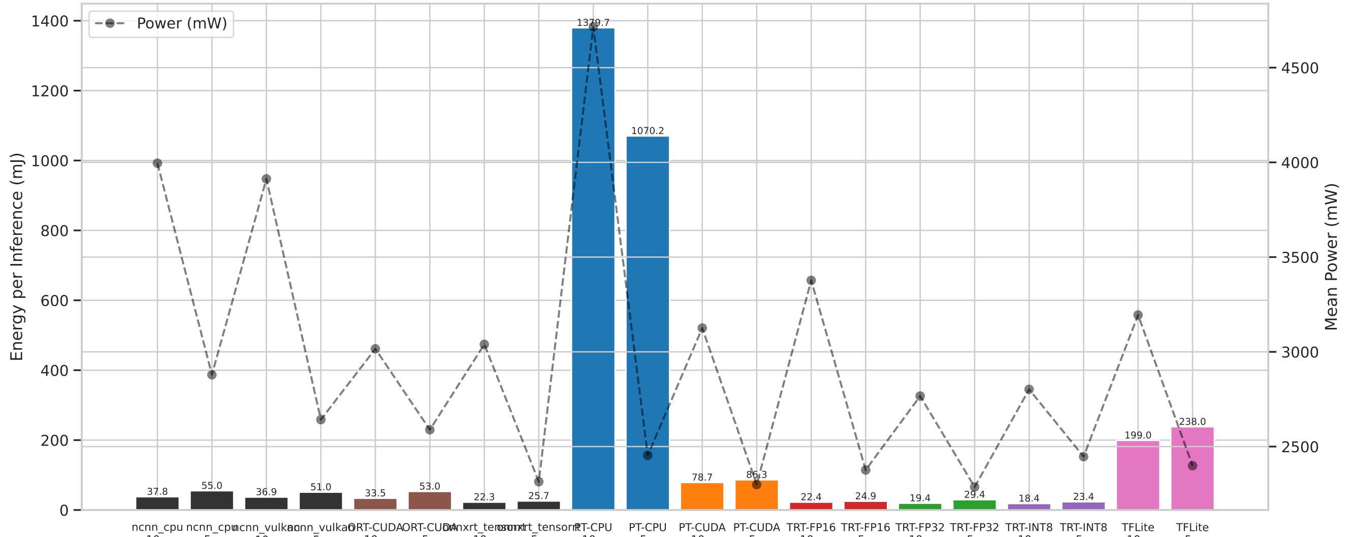
Energy Consumption per Inference: model
