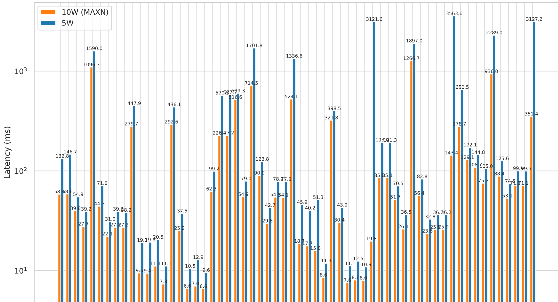
5W vs 10W Mode: Inference Latency Comparison
