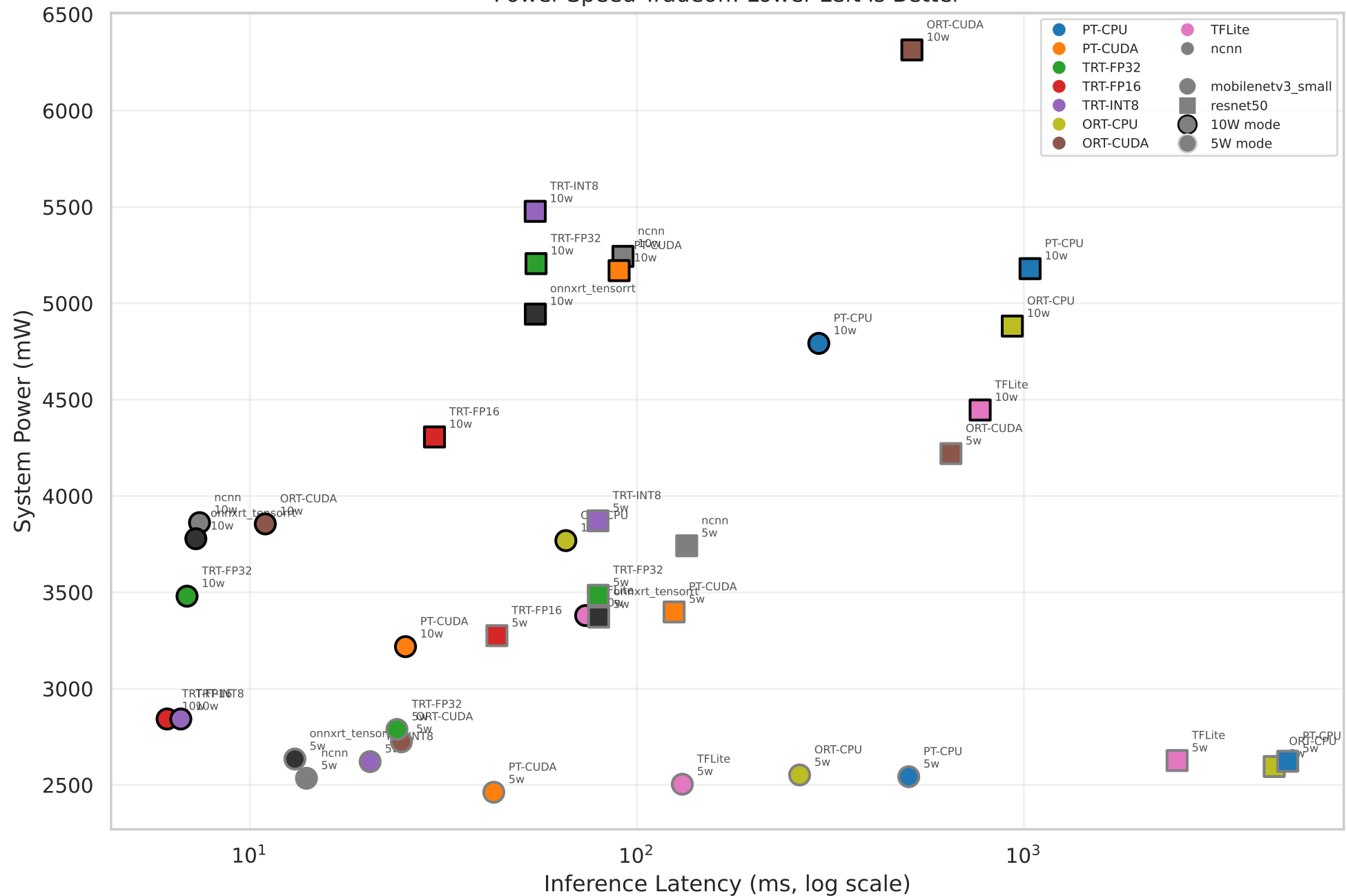
Power-Speed Tradeoff: Lower-Left is Better
