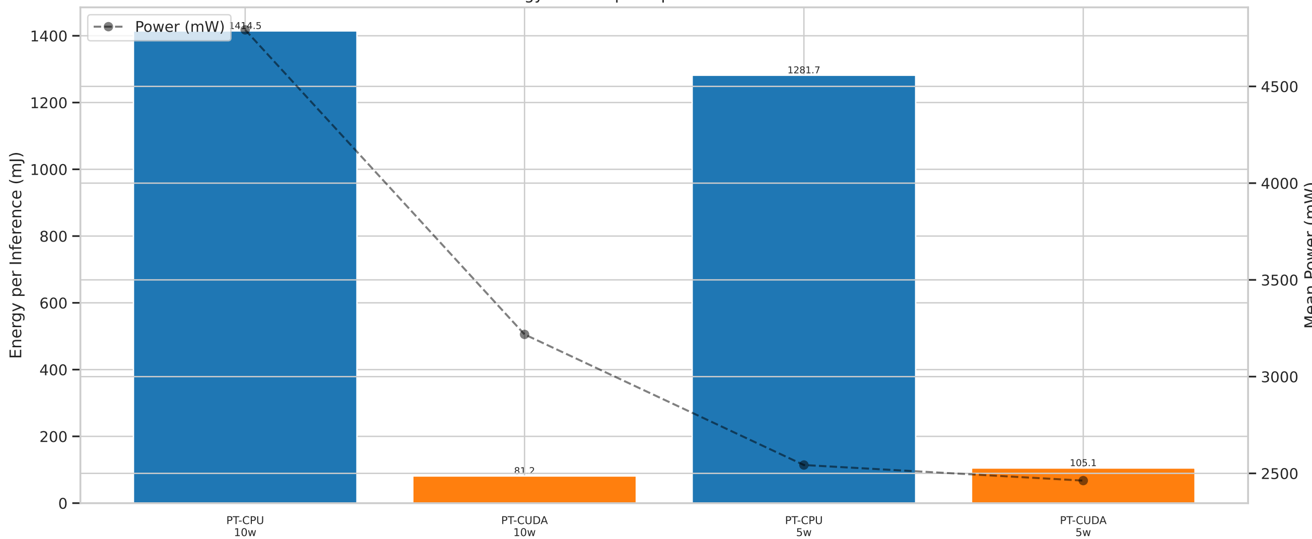
Energy Consumption per Inference: resnet50
