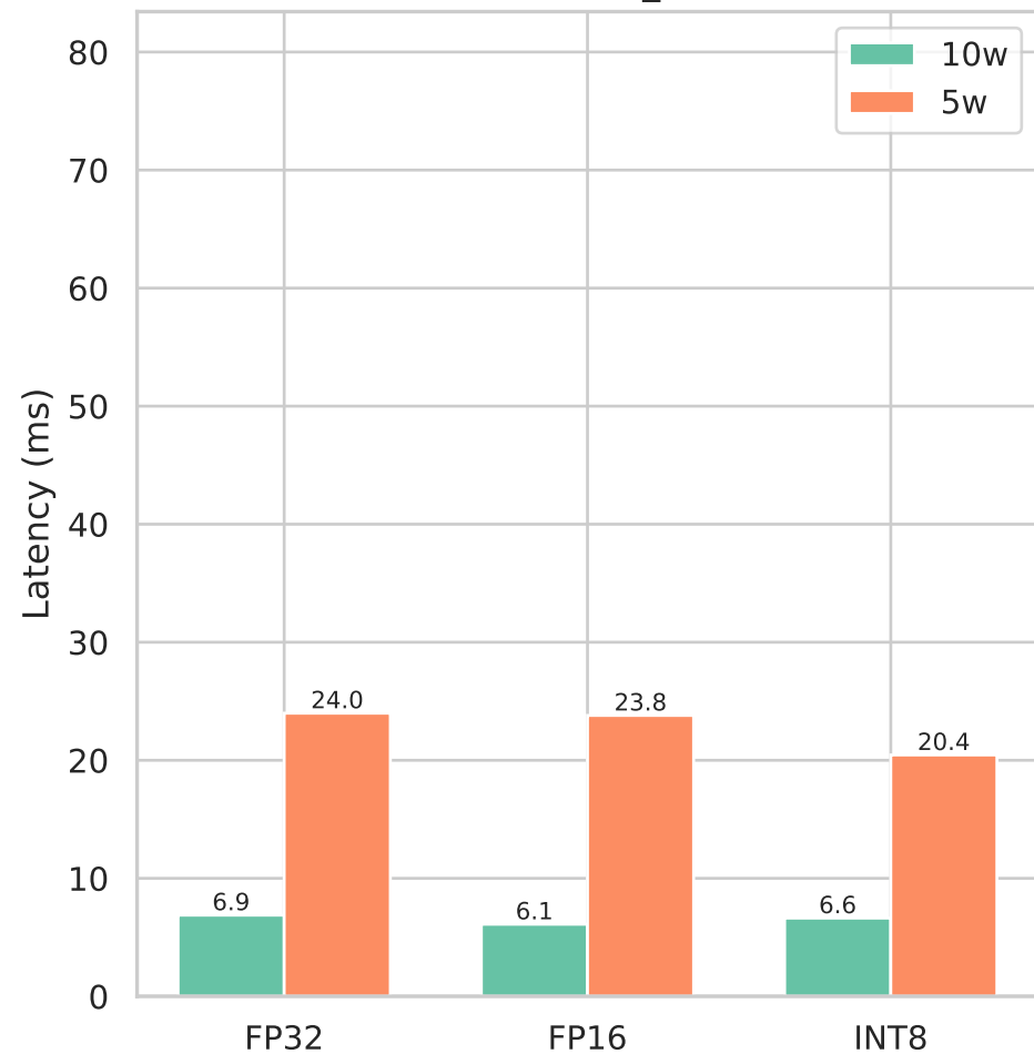
mobilenetv3_small
