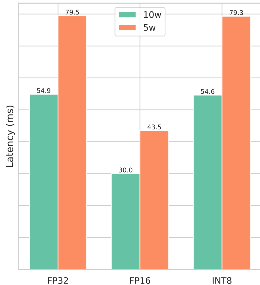
resnet50
