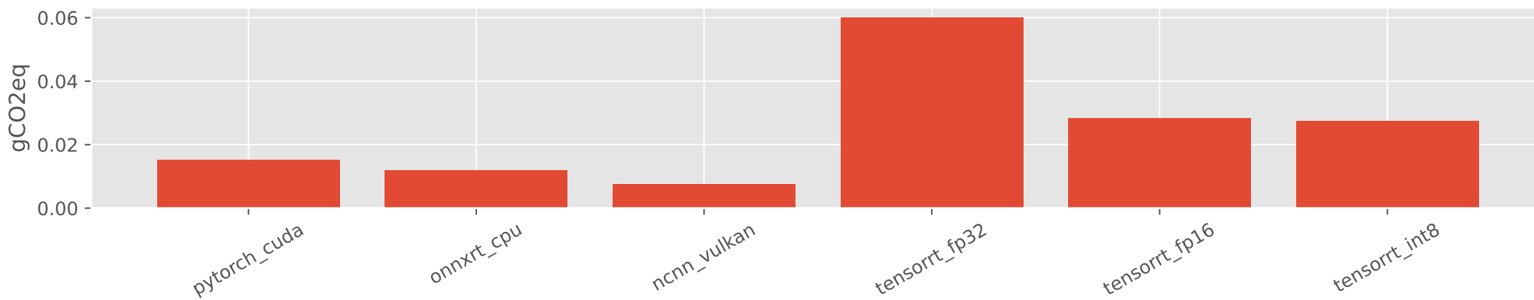
resnet50
