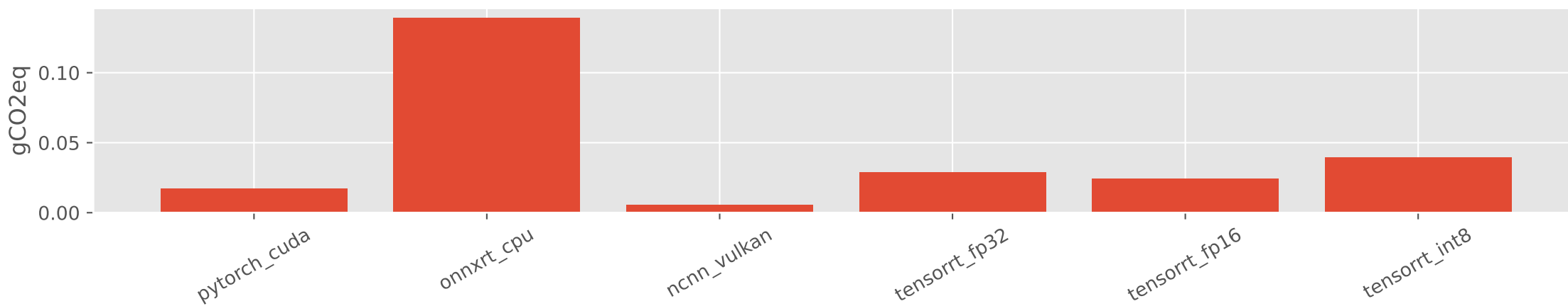
shufflenetv2
