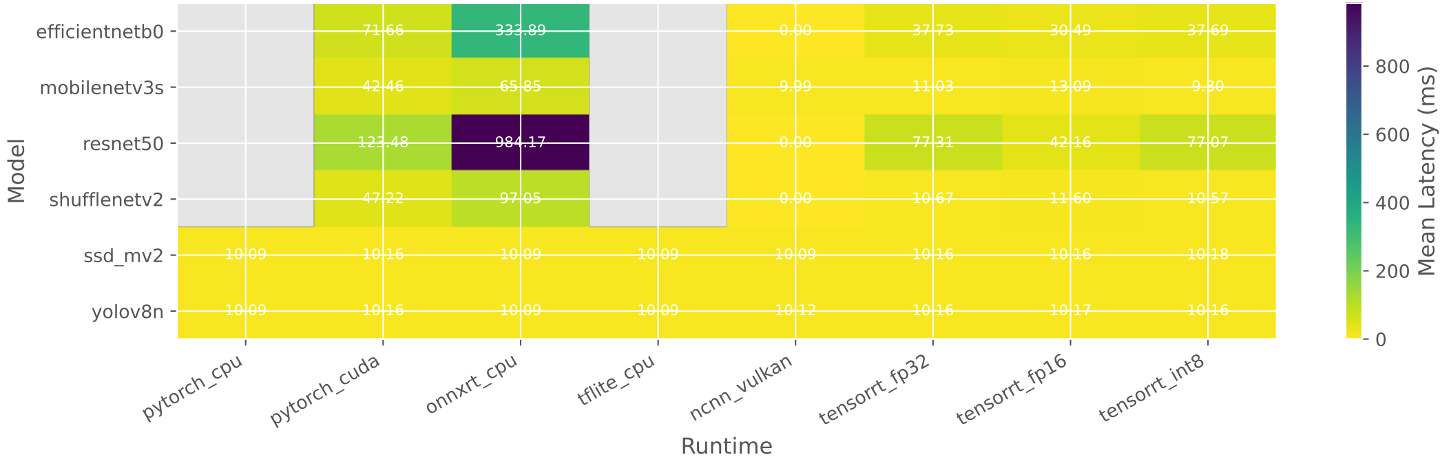
Mean Latency by Model and Runtime
