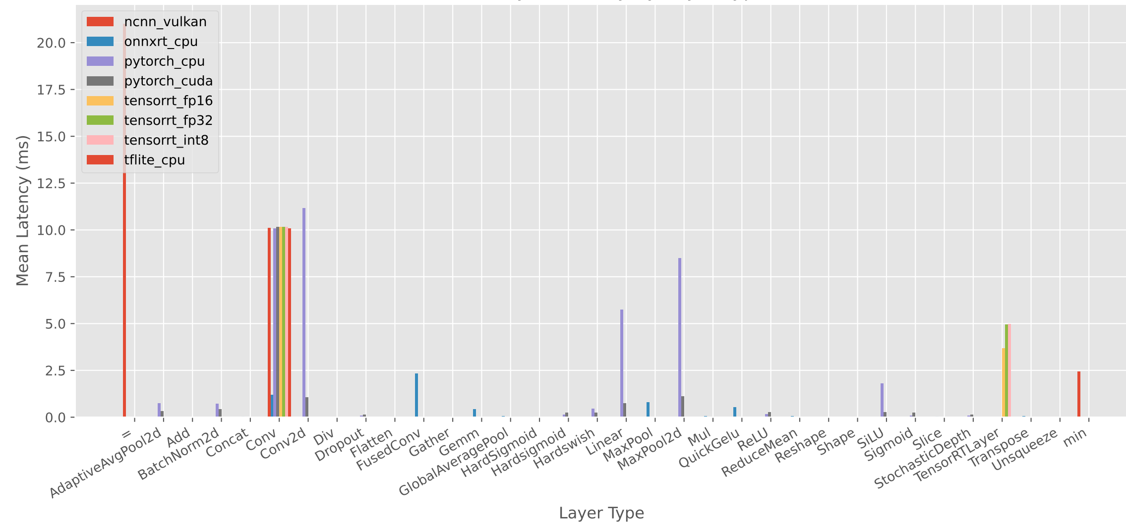
Mean Layer Latency by Layer Type
