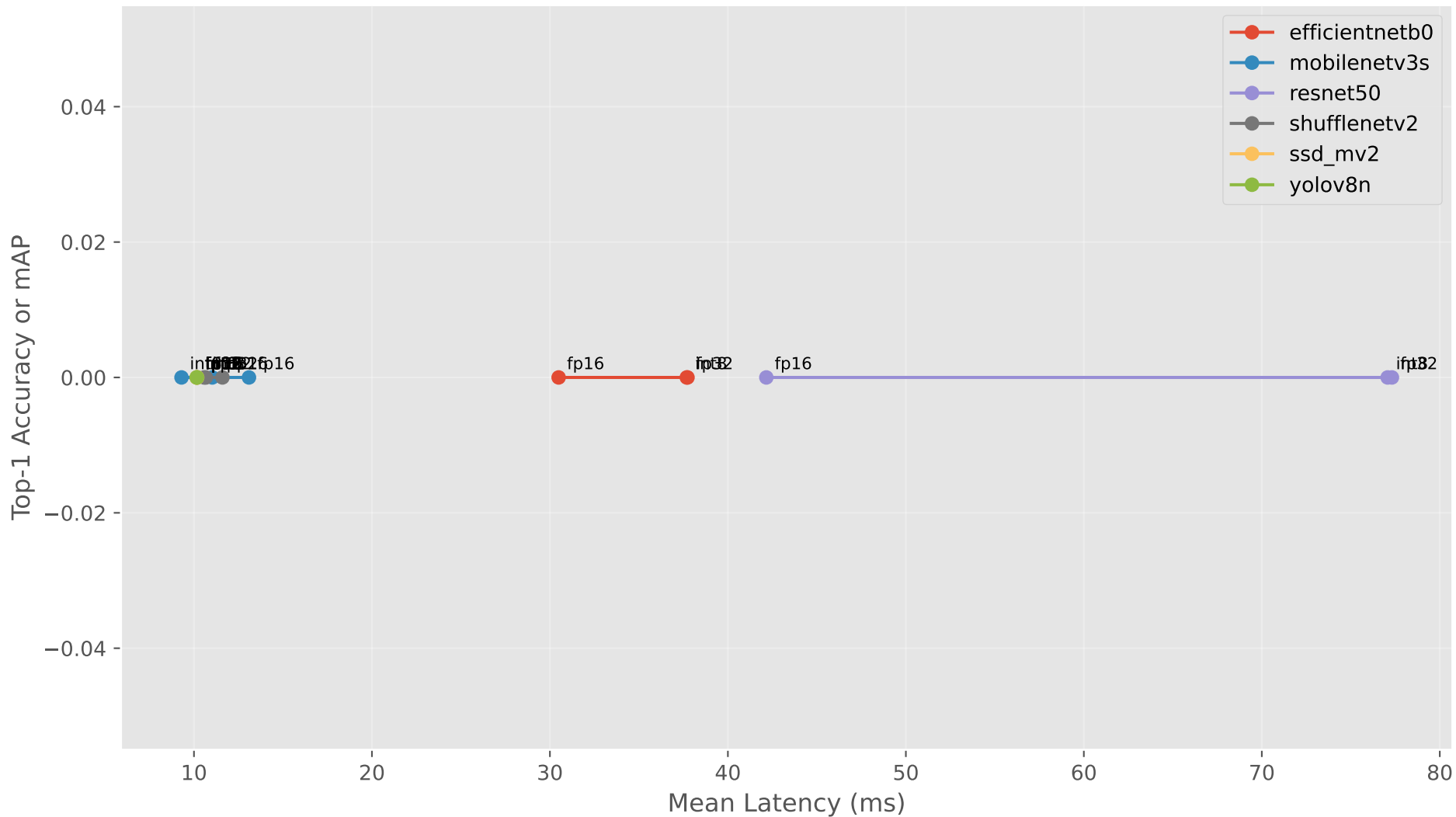
TensorRT Accuracy-Efficiency Curve
