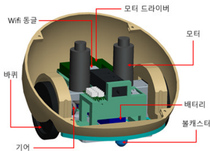
Drive-system packaging
