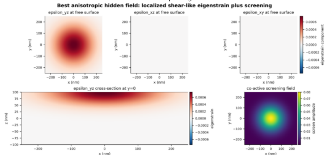
best low-rank anisotropic eigenstrain field
