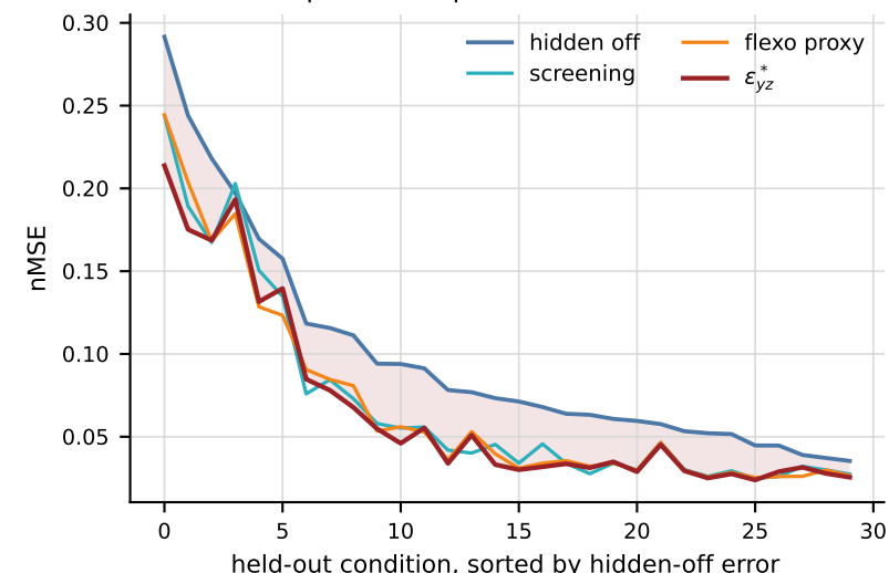
anisotropic field improves all 30 holdout cases
