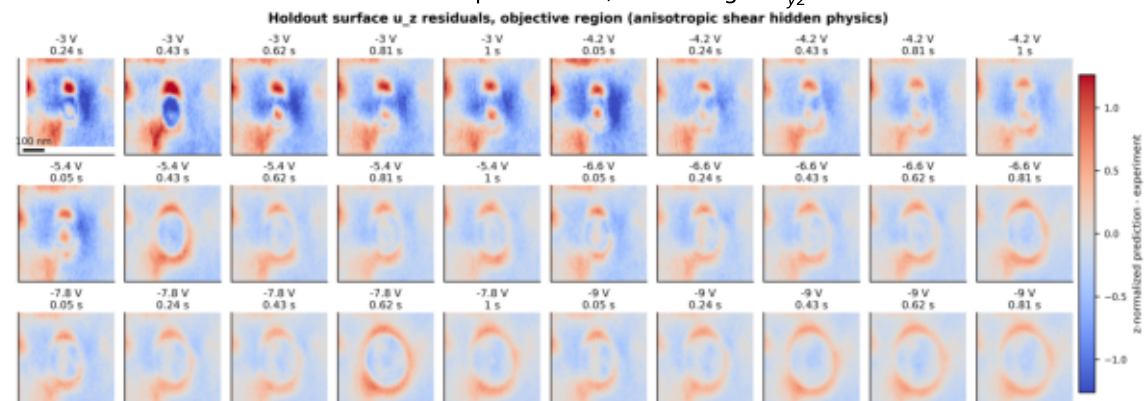
center-crop residuals, screening + \epsilon_{yz}^*
