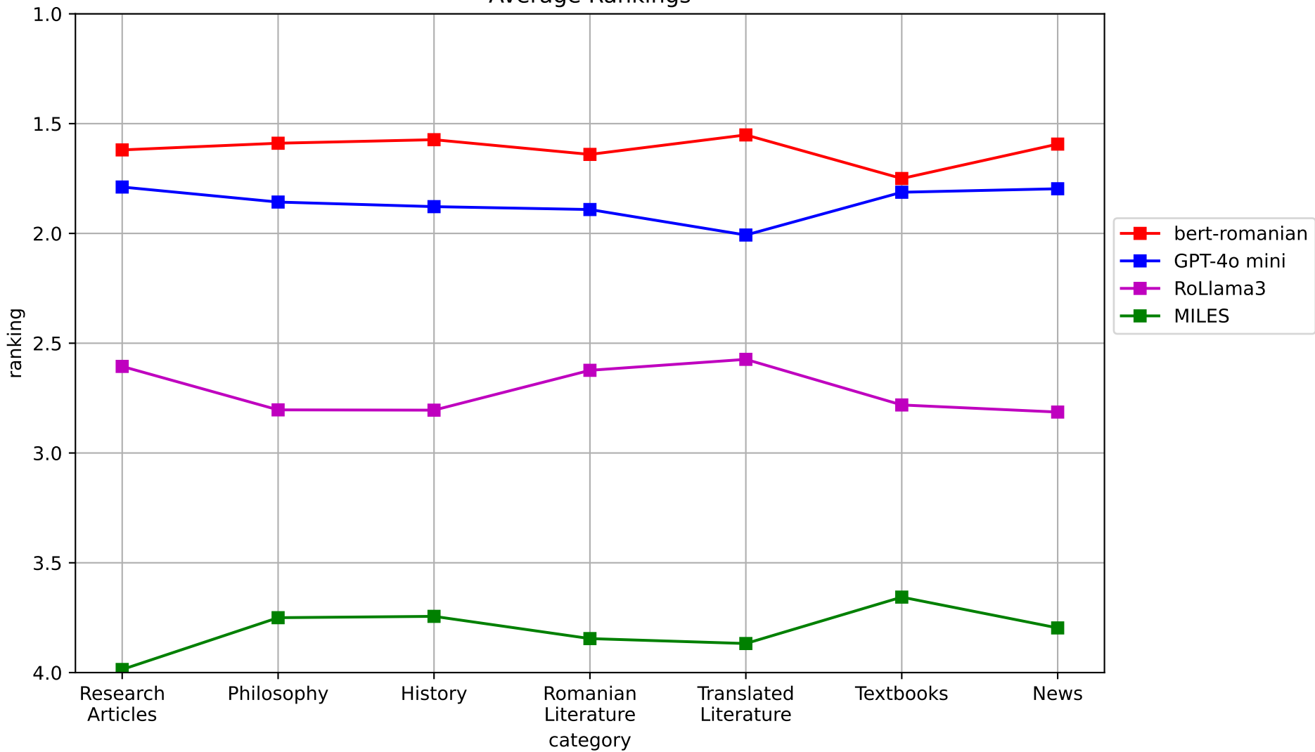
Average Rankings
