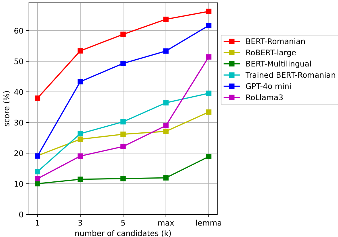
Accuracy@k@top1
