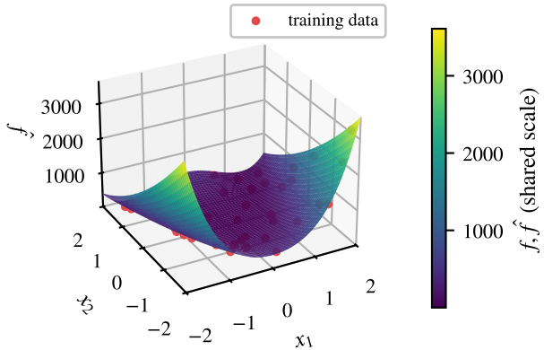
GP \hat{f}
