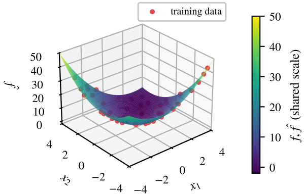
GP \hat{f}
