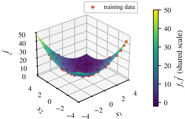
Cubic RBF \hat{f}
