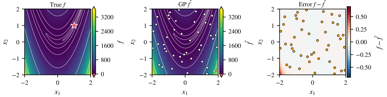
Fig. 7 Rosenbrock, GP surrogate: true f , surrogate \hat{f} with identical color limits, and error f - \hat{f} (diverging scale centered at zero, maximum |e| = 0.699 in the corner (-2, -2) ), with training points overlaid on the surrogate and error panels.
