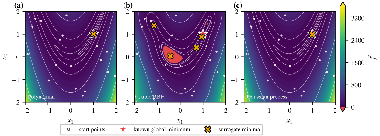
Fig. 12 Rosenbrock: multi-start optimization on (a) the degree-4 polynomial, (b) the cubic RBF and (c) the GP. The background is each surrogate \hat{f} with the color limits of the true function and white iso-lines of \hat{f} ; white dots are the 20 start points, crosses the distinct surrogate minima, and the star the known global minimum. Four distinct RBF minima were found from the 20 starts, including the spurious deepest one at (-0.44, 0.04) , which lies inside the large red region where \hat{f} < -3.6 . The small red patch near (1.2, 1.45) is a further undershoot that no start reached.
