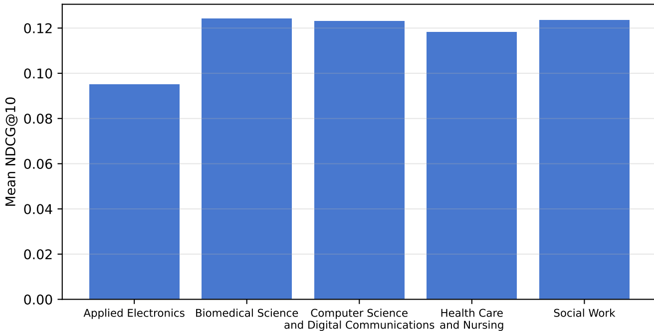
GraphSAGE recommendation quality per study-path cohort
