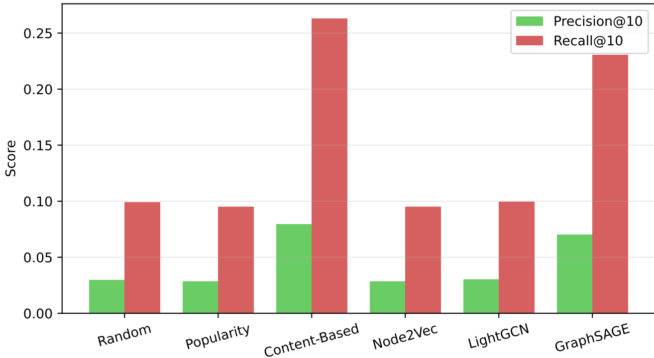
Precision@10 and Recall@10 on cold-start users
