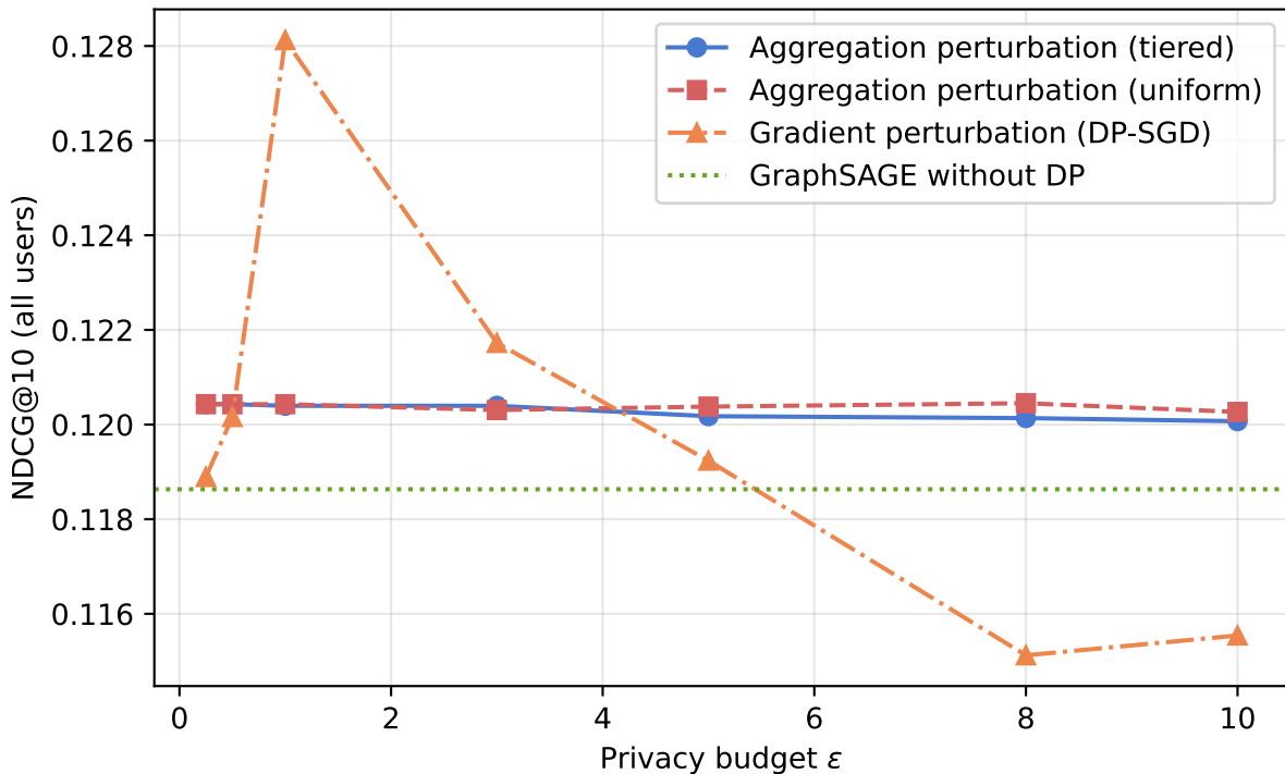
Privacy-utility trade-off
