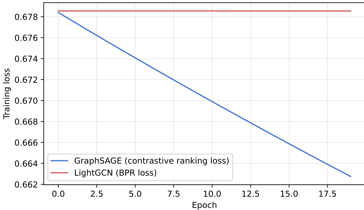
Training convergence
