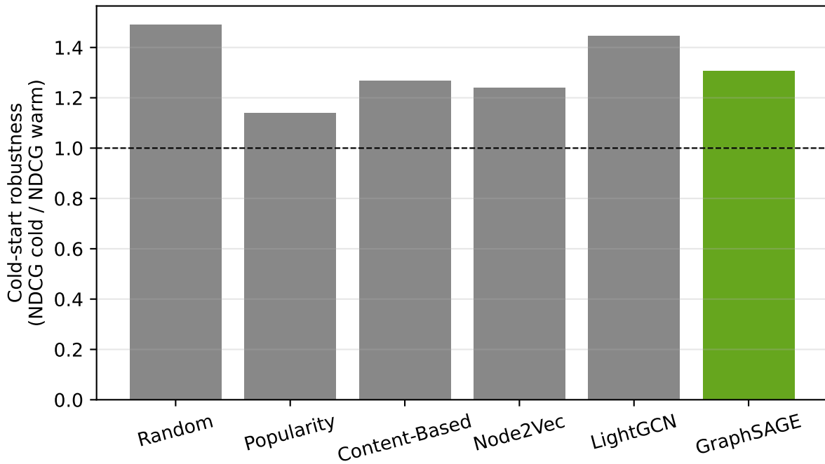
Cold-start robustness by model
