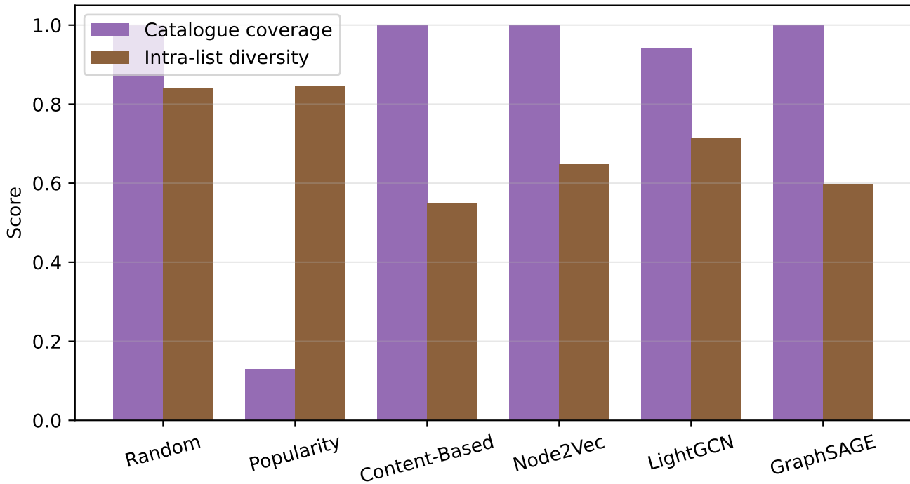
Beyond-accuracy metrics (top-10 lists)
