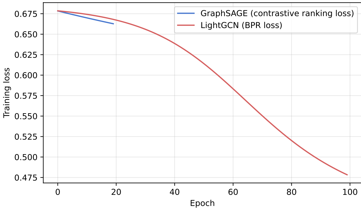
Training convergence
