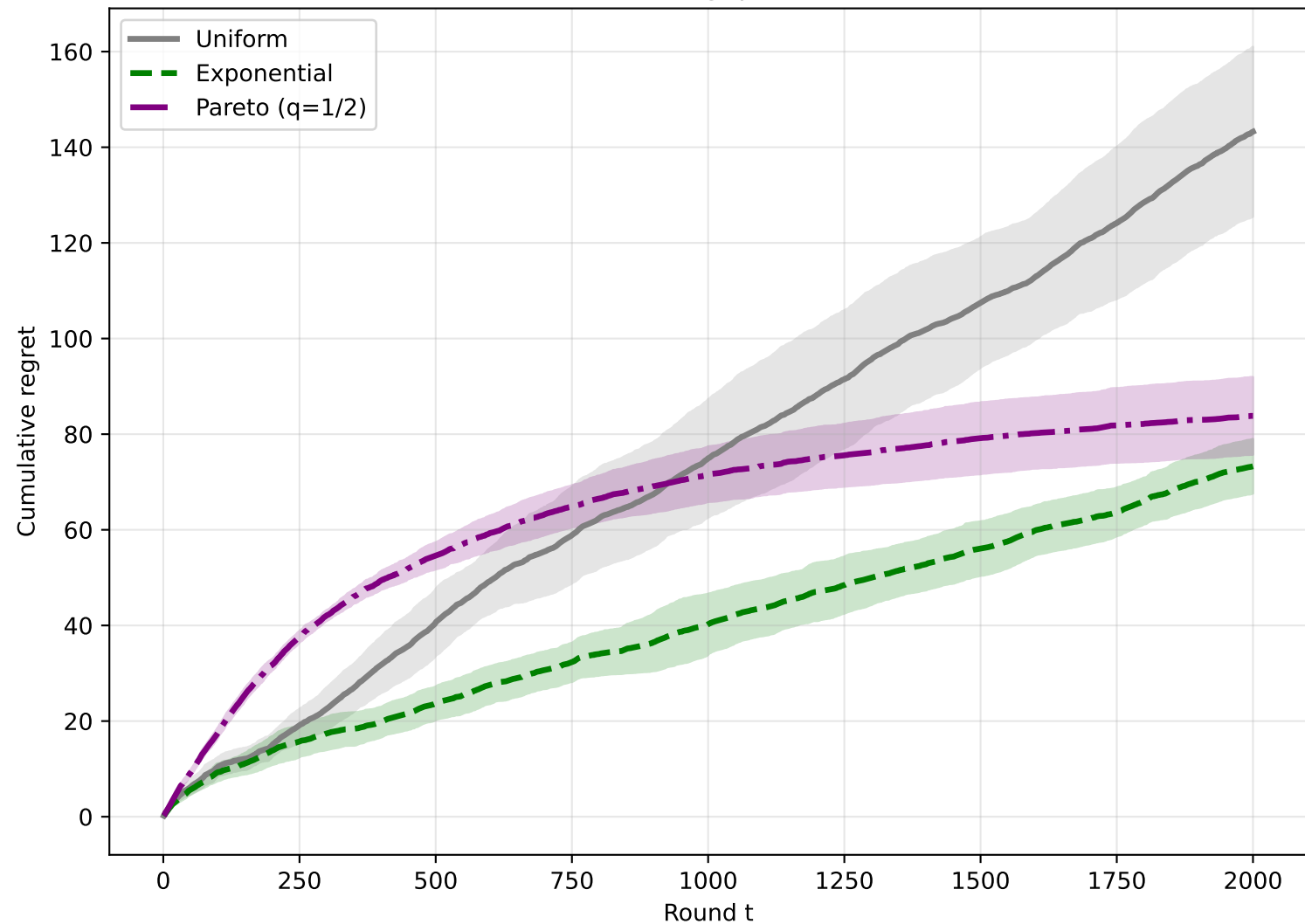
Stochastic, K=5 , \text{gap}=0.1 , T=2000
