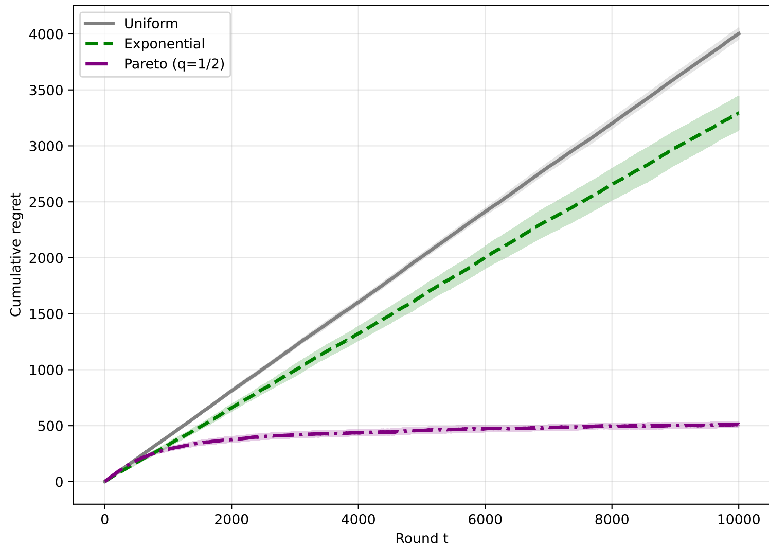
Adversarial, K=20 , T=10000
