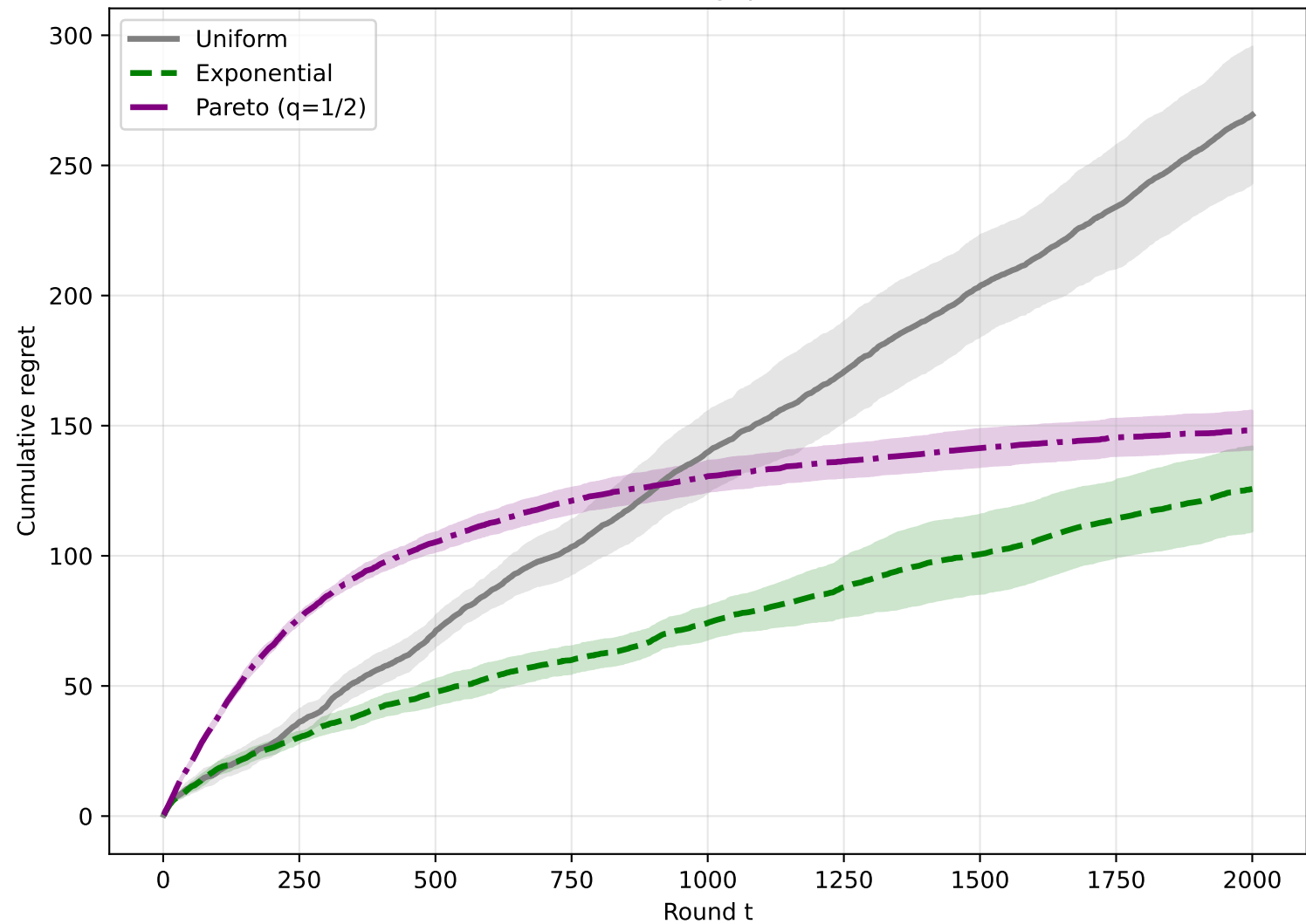
Stochastic, K=10 , \text{gap}=0.1 , T=2000
