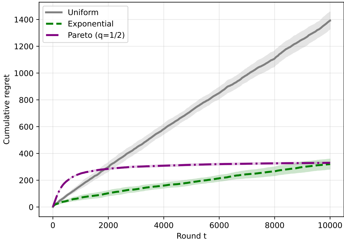
Stochastic, K=10 , \text{gap}=0.2 , T=10000
