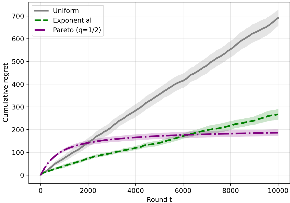
Stochastic, K=5 , \text{gap}=0.1 , T=10000
