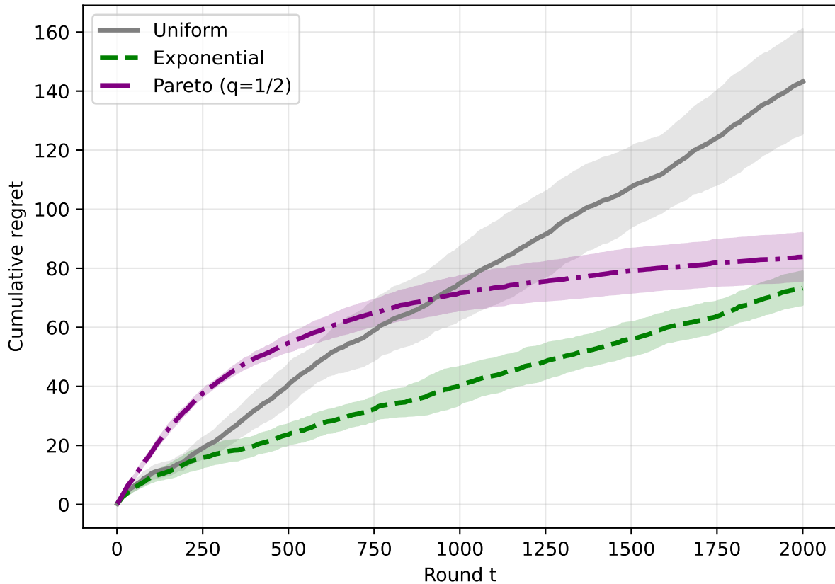
Stochastic, K=5 , \text{gap}=0.1 , T=2000
