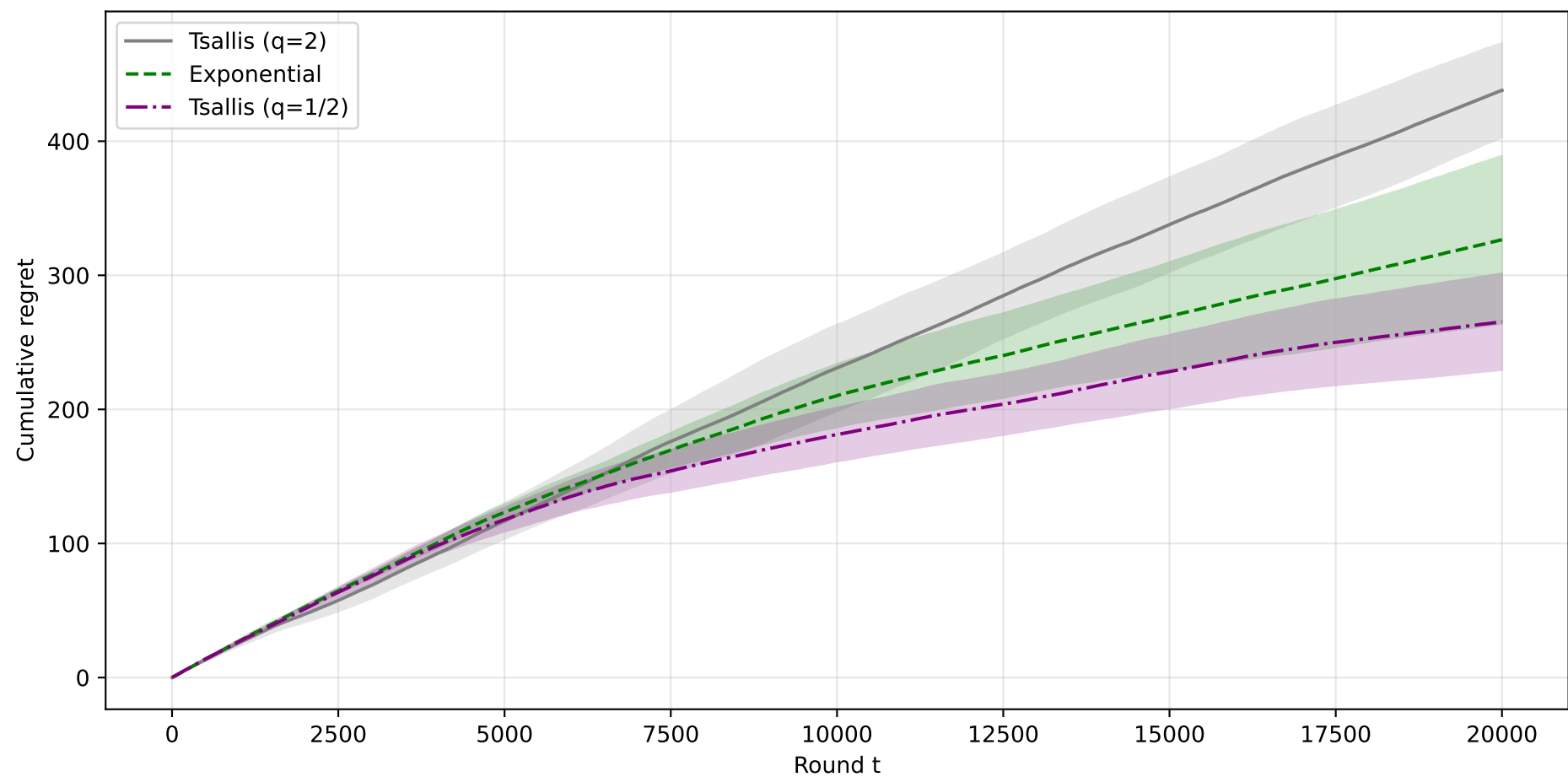
Stochastic environment
