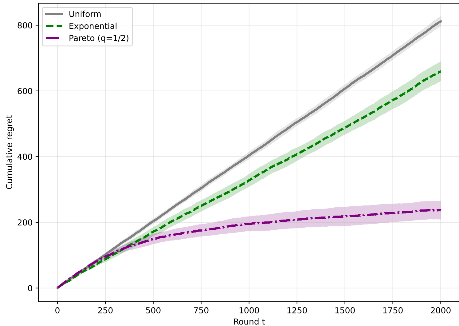
Adversarial, K=20 , T=2000
