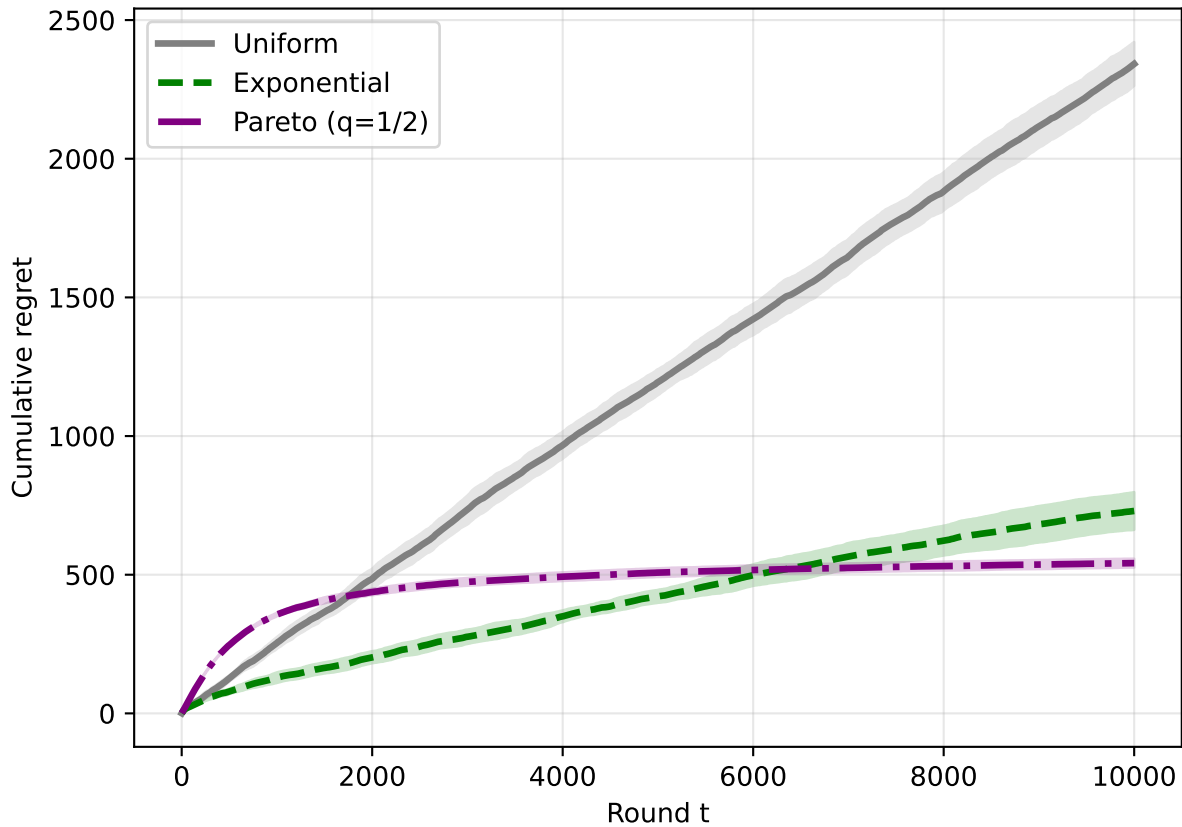
Stochastic, K=20 , \text{gap}=0.1 , T=10000
