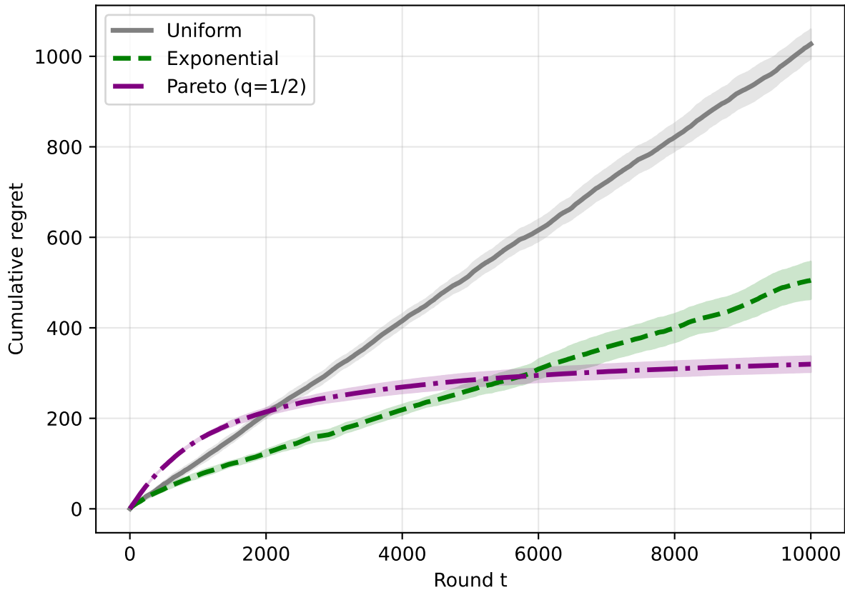
Stochastic, K=10 , \text{gap}=0.05 , T=10000
