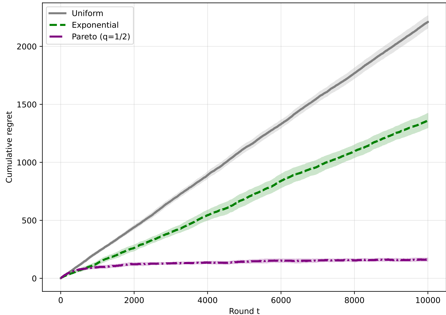
Adversarial, K=5 , T=10000
