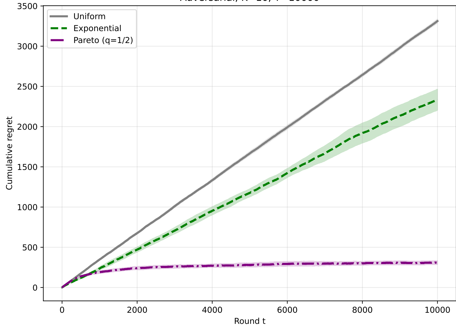
Adversarial, K=10 , T=10000
