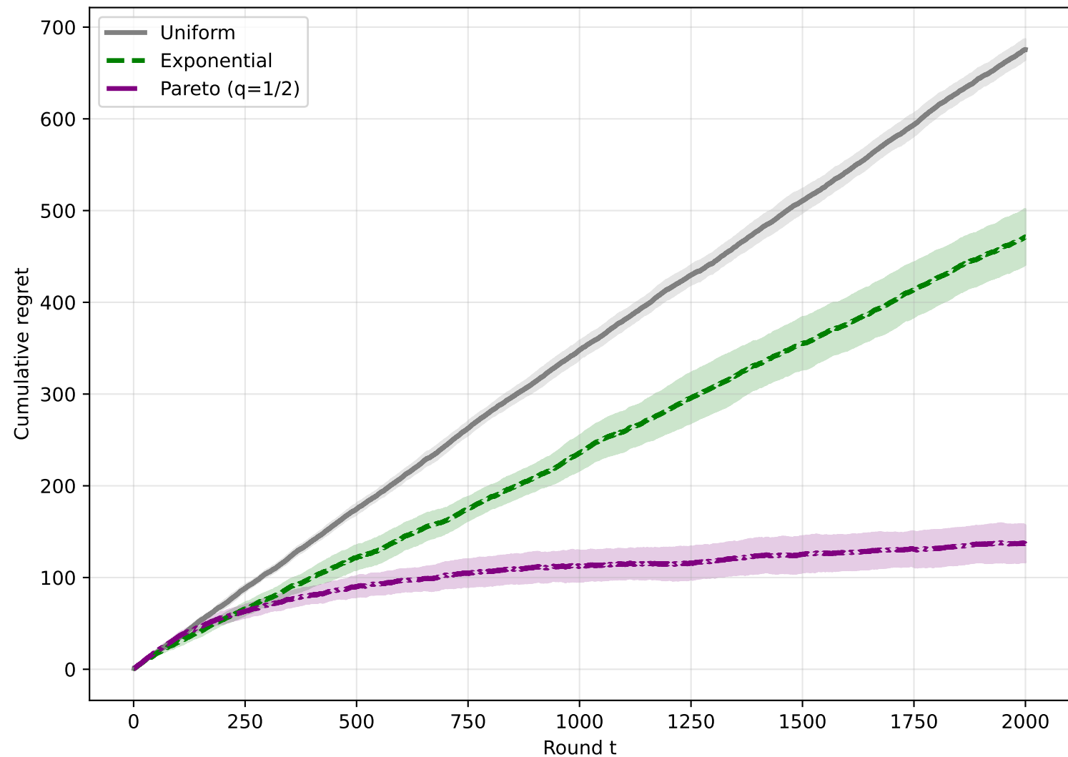
Adversarial, K=10 , T=2000
