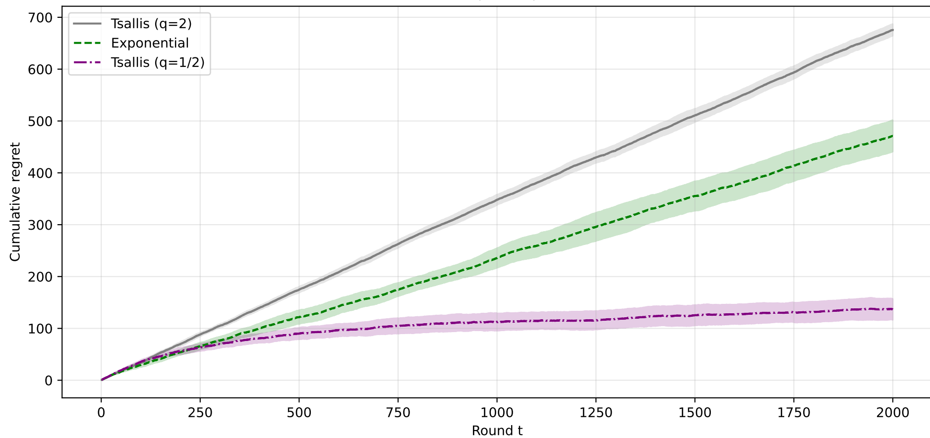
Adversarial, K=10 , T=2000
