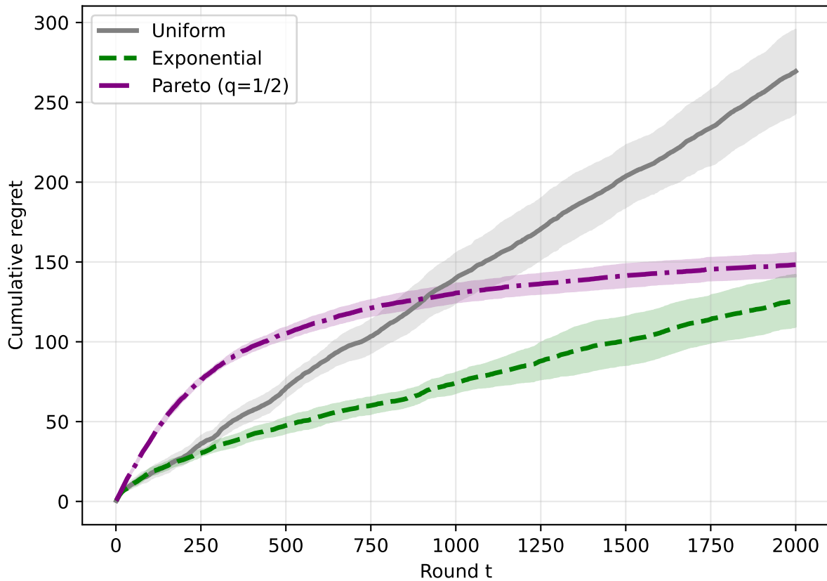
Stochastic, K=10 , \text{gap}=0.1 , T=2000
