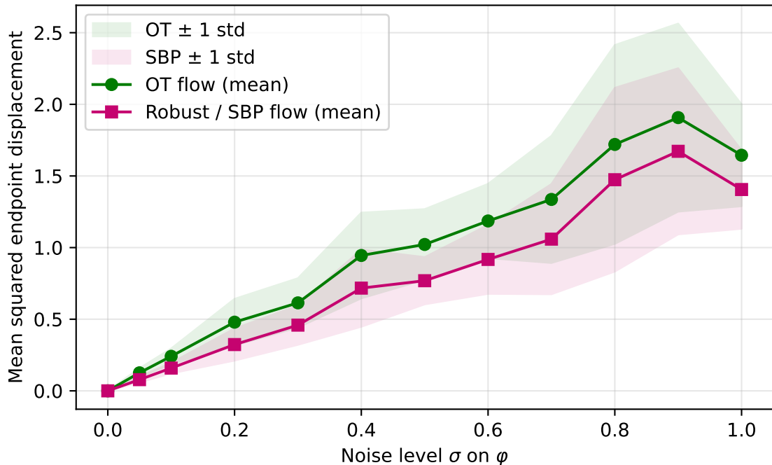
Endpoint sensitivity vs potential noise averaged over 10 runs
