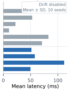
(c) Latency
