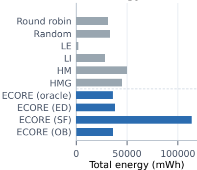
(a) Energy
