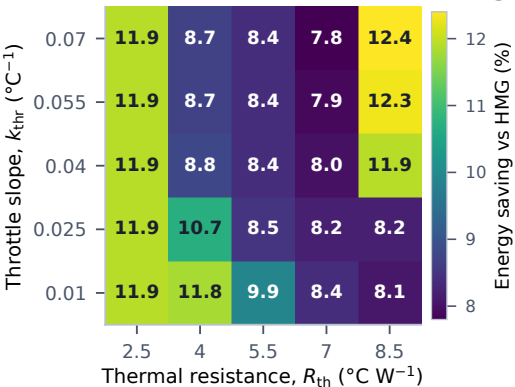
(a) Thermal model: headline saving
