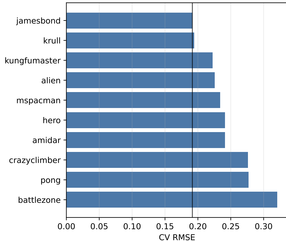
Atari-1 validation candidates
