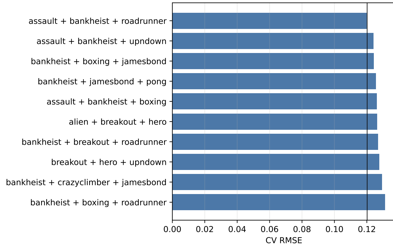
Atari-3 candidates
