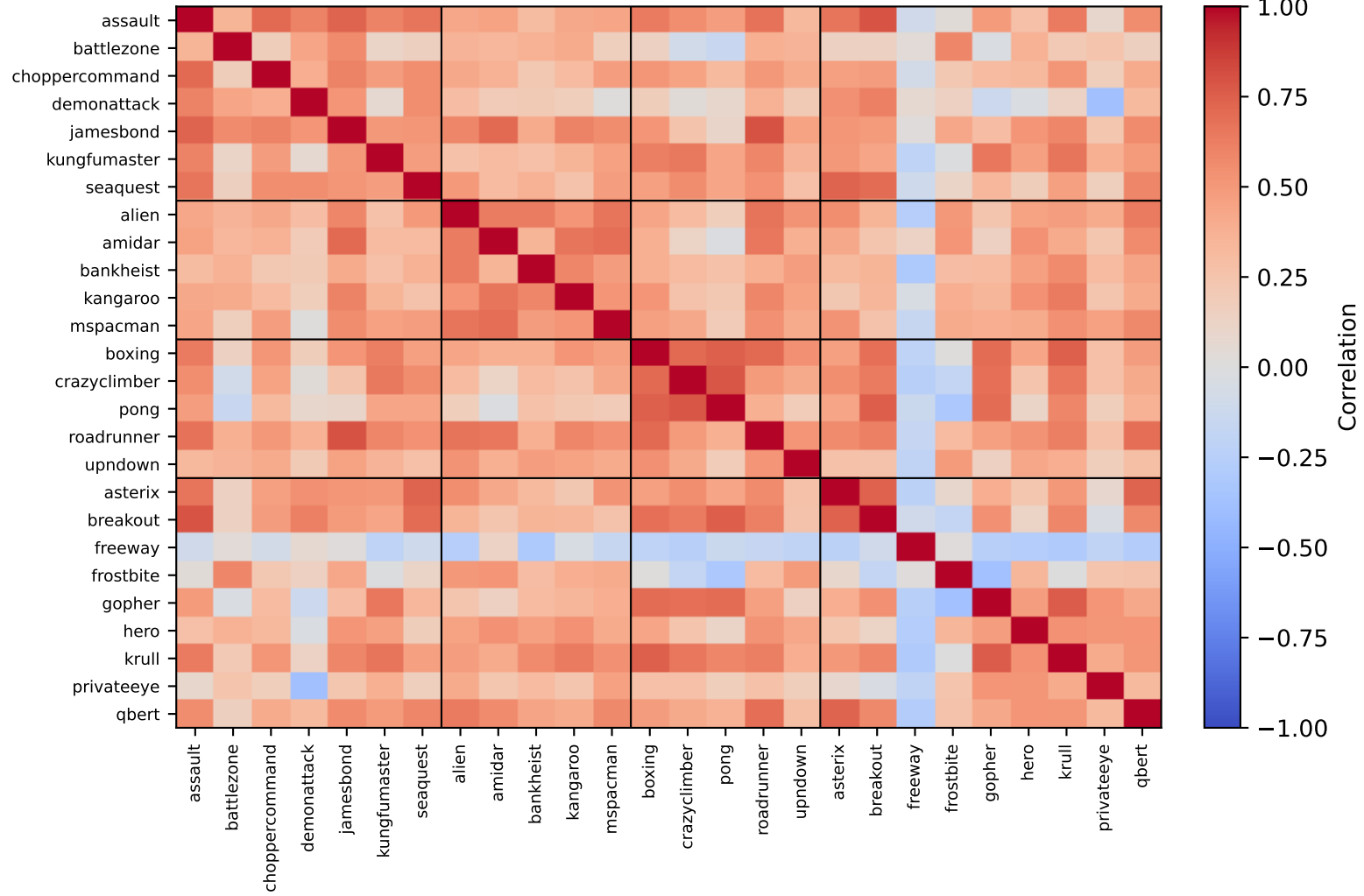
Game correlation across methods Pearson r of log-HNS Combat Maze Sports Action
