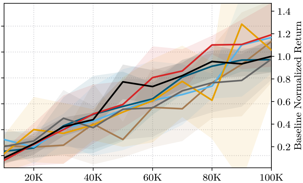
Environment Steps
