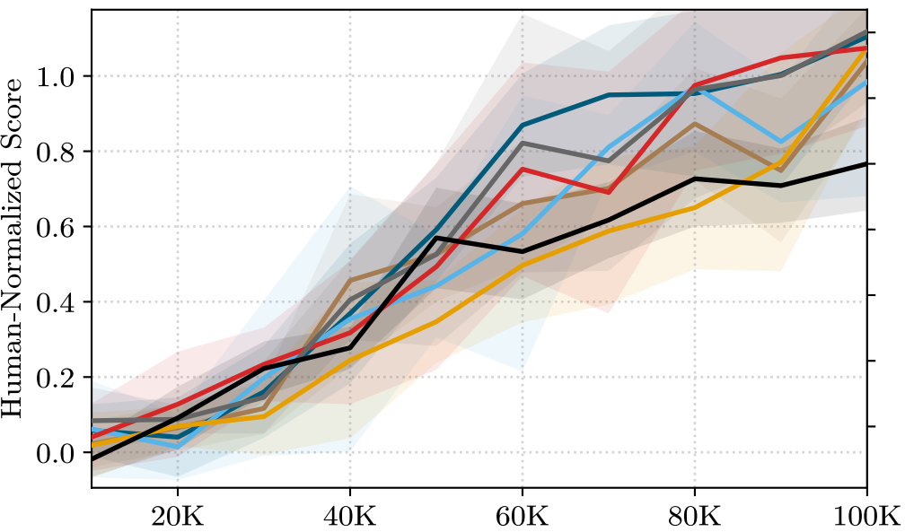
Environment Steps
