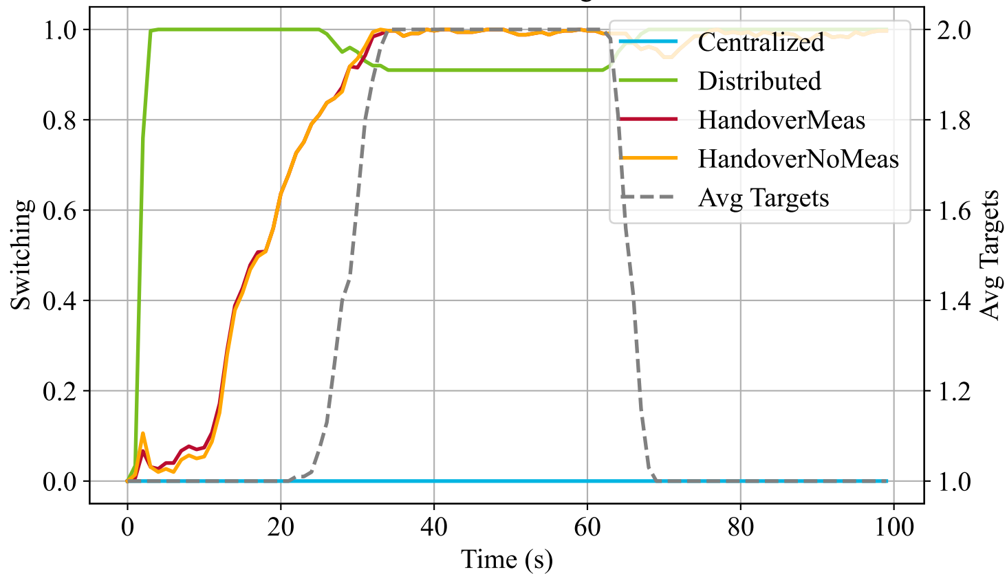
BS2: Switching
