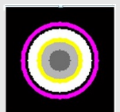
Initialization
