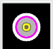
Level Set
