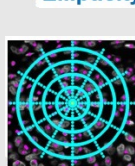
Angular Histogram
