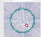
Diffusion with Dirichlet boundary condition
