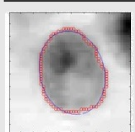
Normal Cell
