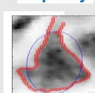
Abnormal Cell
