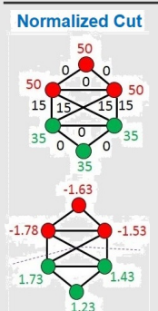
Normalized Cut
