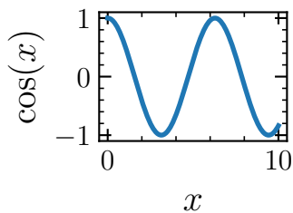
Cosine Function
