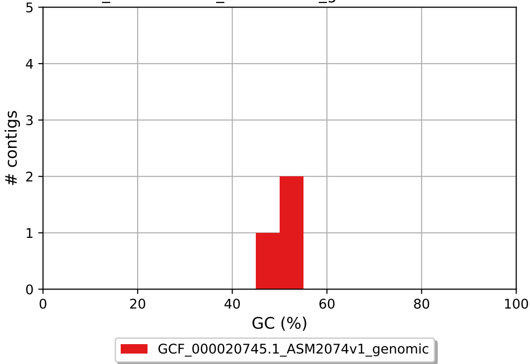
GCF_000020745.1_ASM2074v1_genomic GC content
