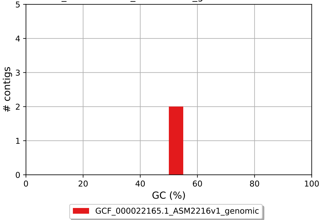
GCF_000022165.1_ASM2216v1_genomic GC content
