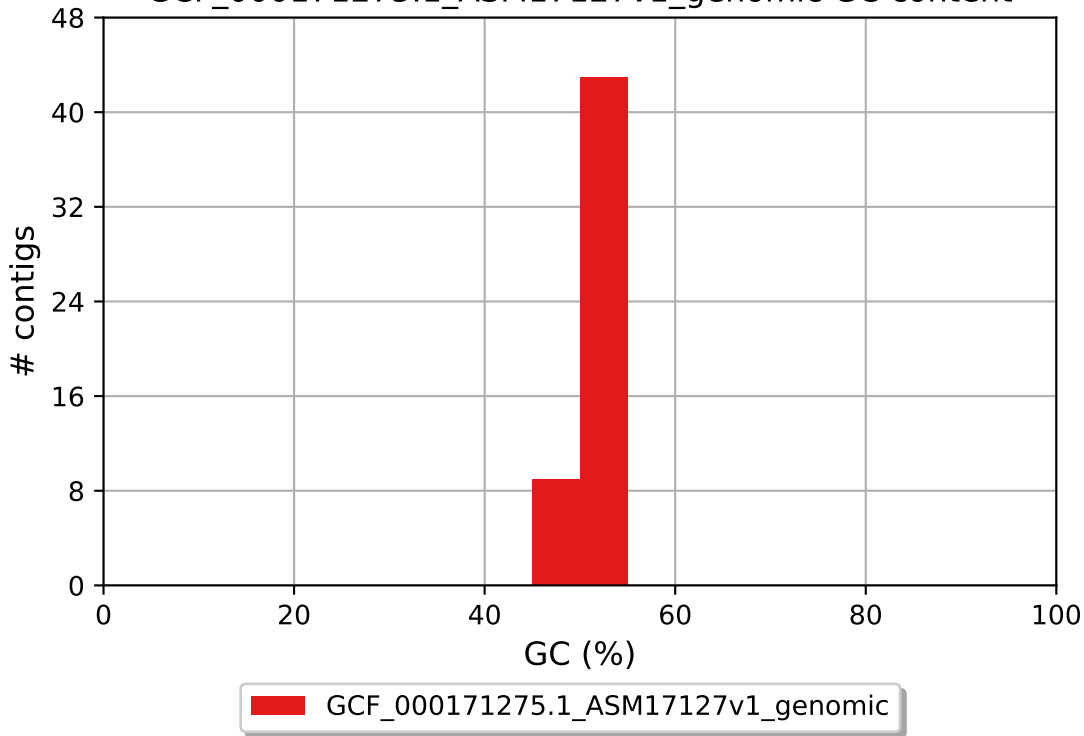
GCF_000171275.1_ASM17127v1_genomic GC content
