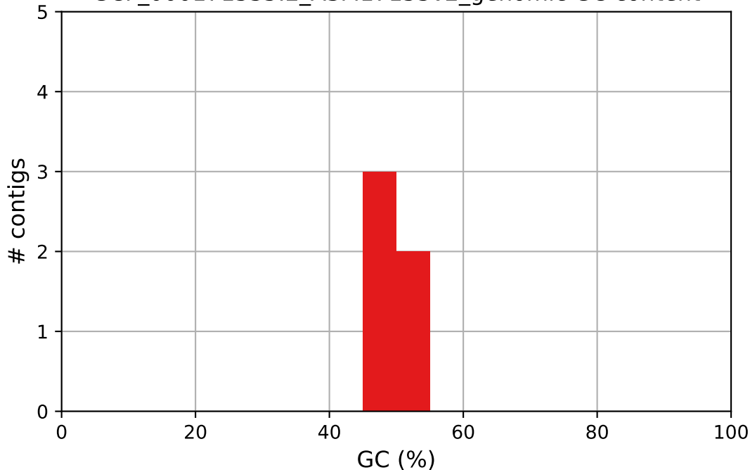
GCF_000171535.2_ASM17153v2_genomic GC content
