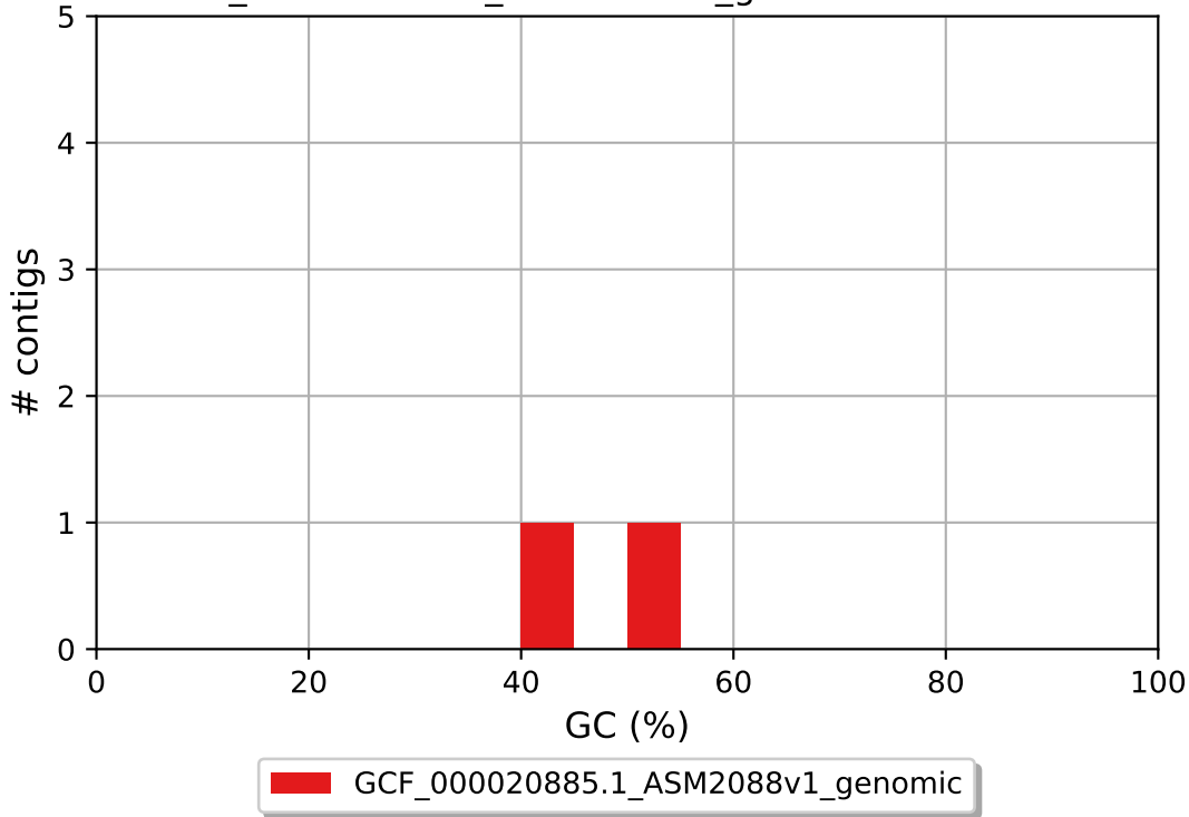
GCF_000020885.1_ASM2088v1_genomic GC content
