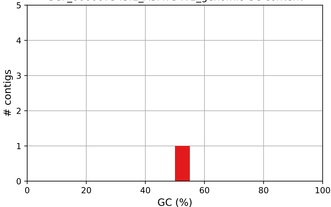
GCF_000007545.1_ASM754v1_genomic GC content
