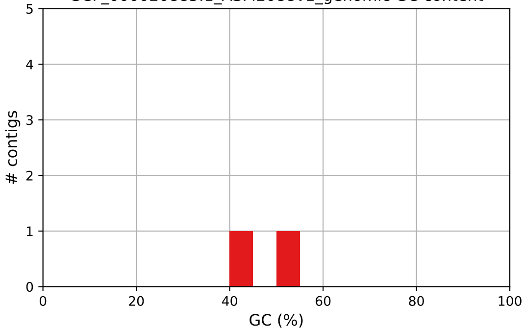
GCF_000020885.1_ASM2088v1_genomic GC content
