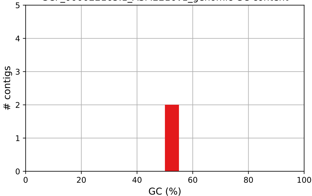
GCF_000022165.1_ASM2216v1_genomic GC content
