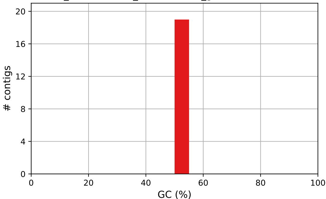
GCF_000171255.1_ASM17125v1_genomic GC content
