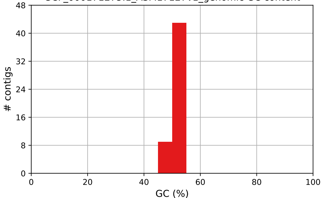
GCF_000171275.1_ASM17127v1_genomic GC content
