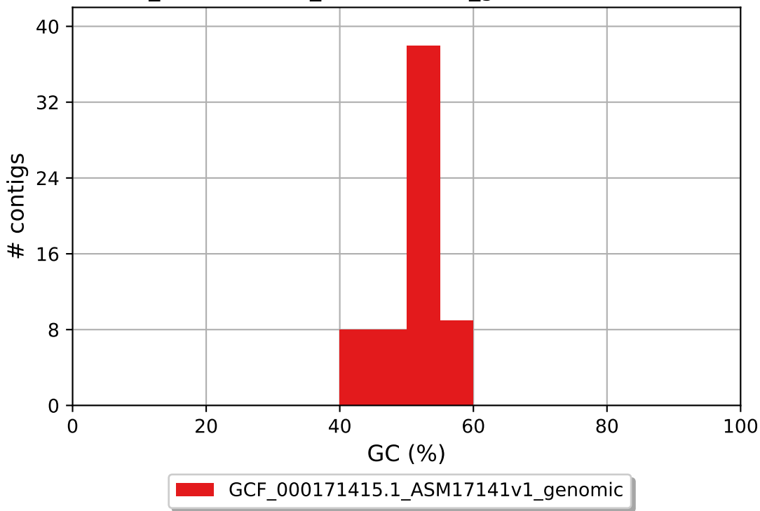
GCF_000171415.1_ASM17141v1_genomic GC content
