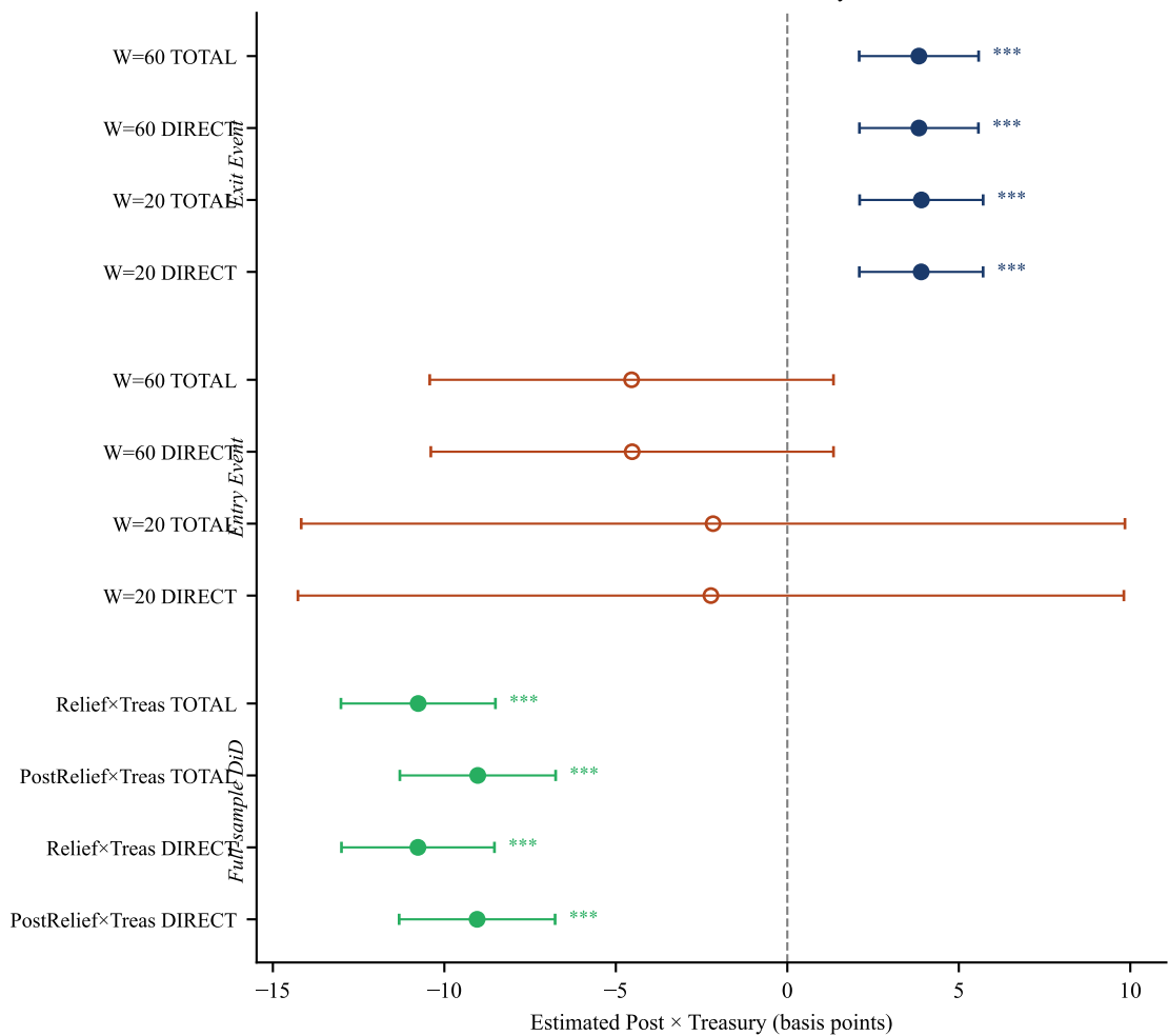
Pooled DiD Estimates: Post \times Treasury Coefficient
