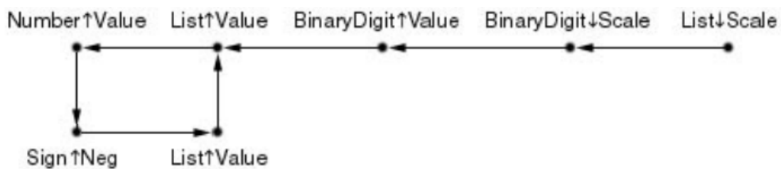
Figure 2.4: Modified attribute dependency graph with circularity
