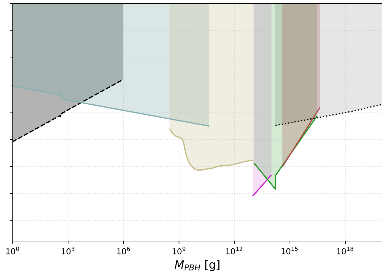
With accretion ( N_{fin} = 30.0, a_* = 0.0, L = 50.3 )
