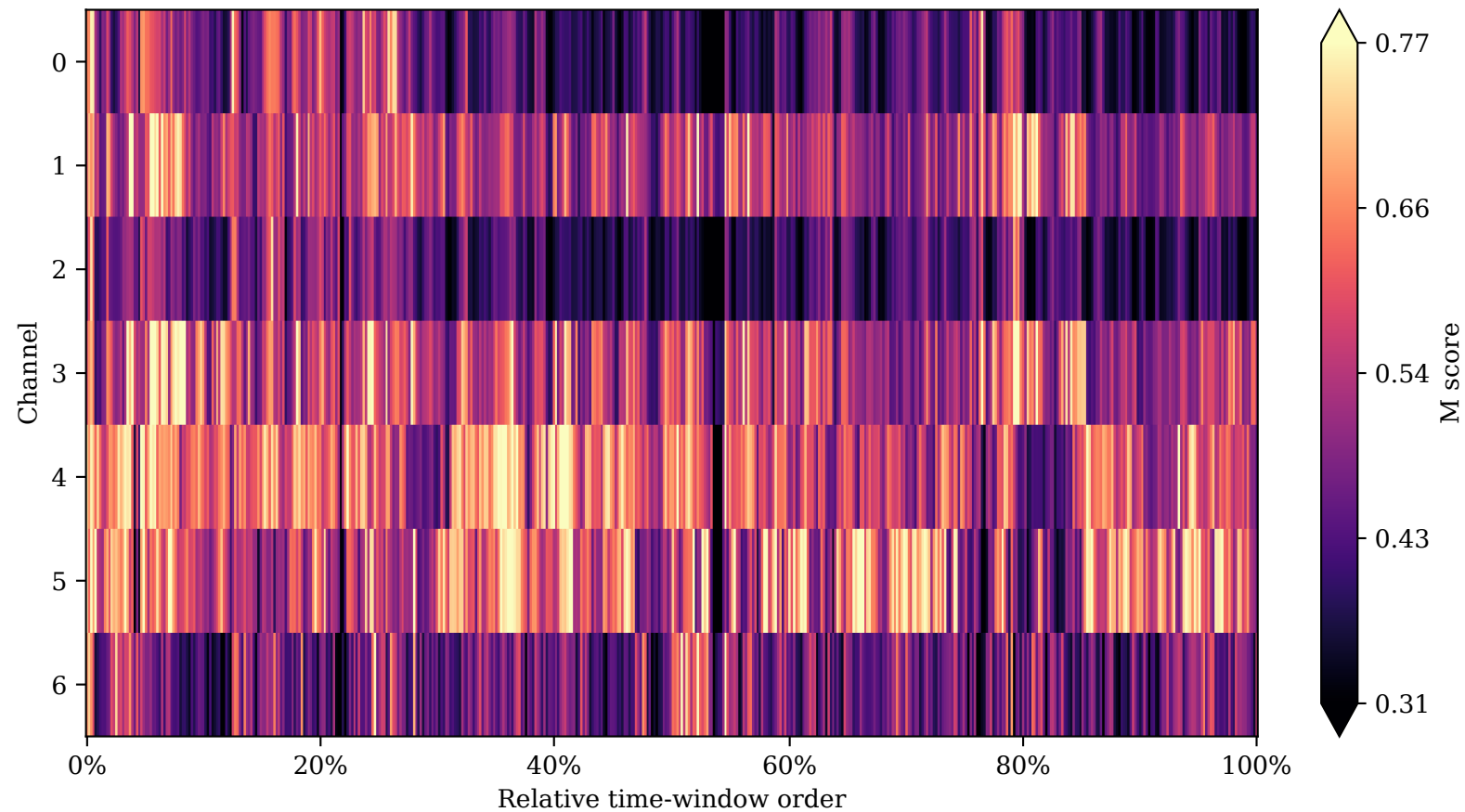
ETTh1: M across channels and time windows
